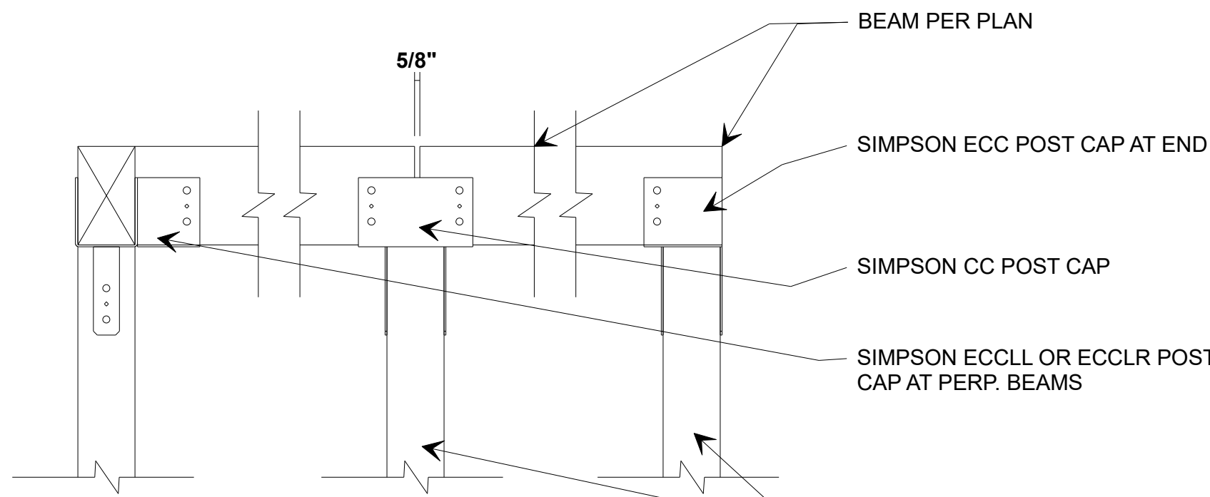
Beam(s) to Post
