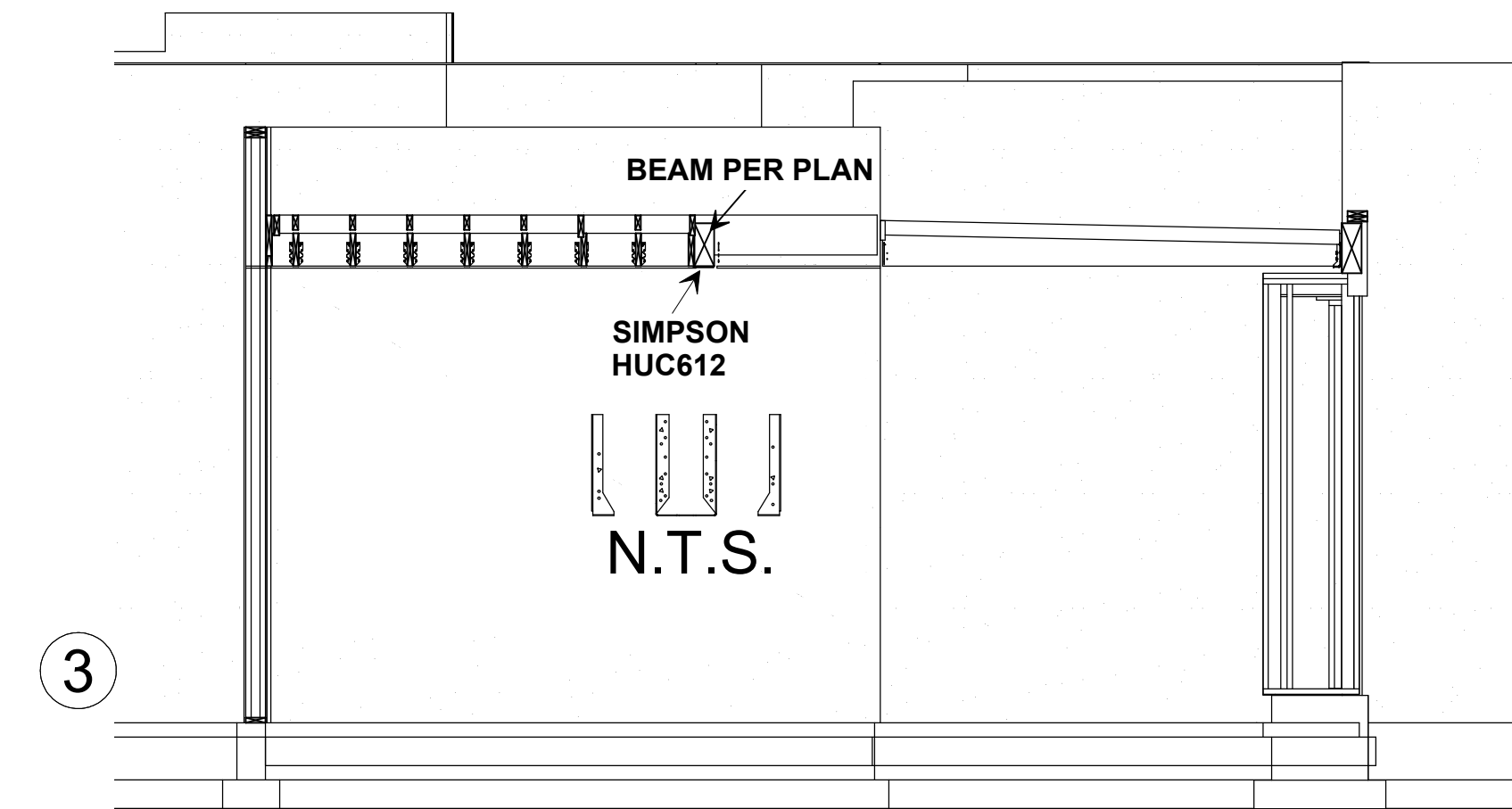
Beam(s) to Post
