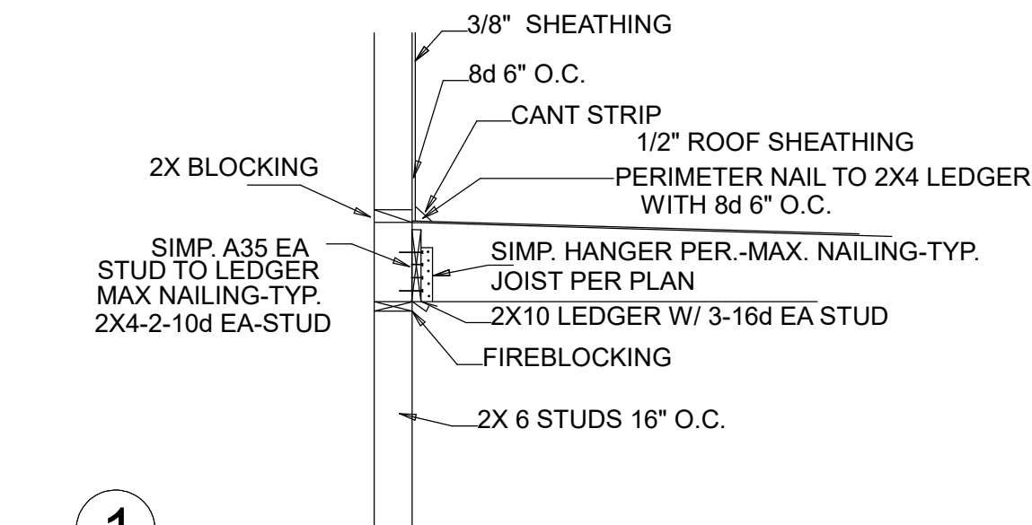
NAIL ON LEDGER
